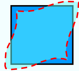
Face Shear Mode
