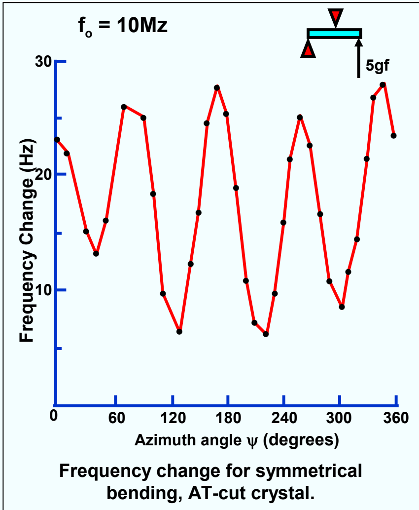
AT-cut resonator
