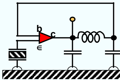
Modified Butler
