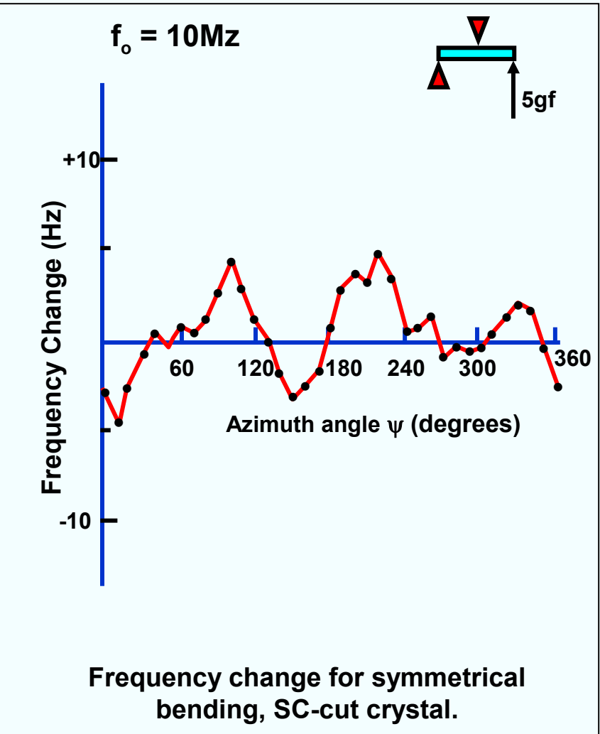
SC-cut resonator
