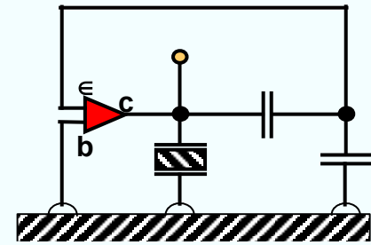
Clapp
