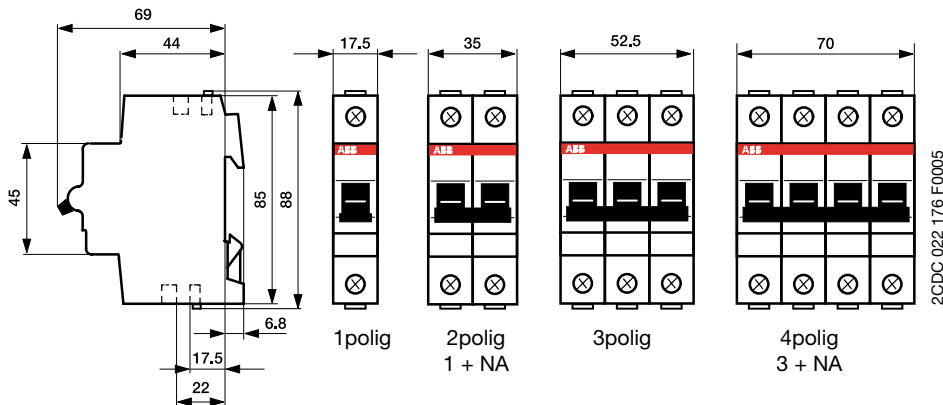
S2C-CM
