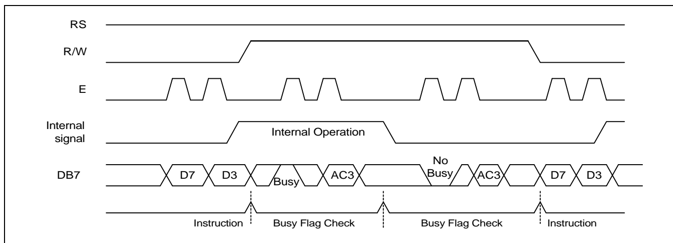
Fig 18. Example of 4-bit Bus Mode Timing Sequence
