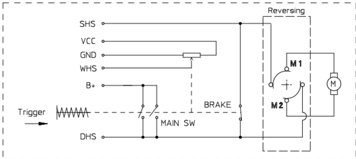
Circuit Schematic
