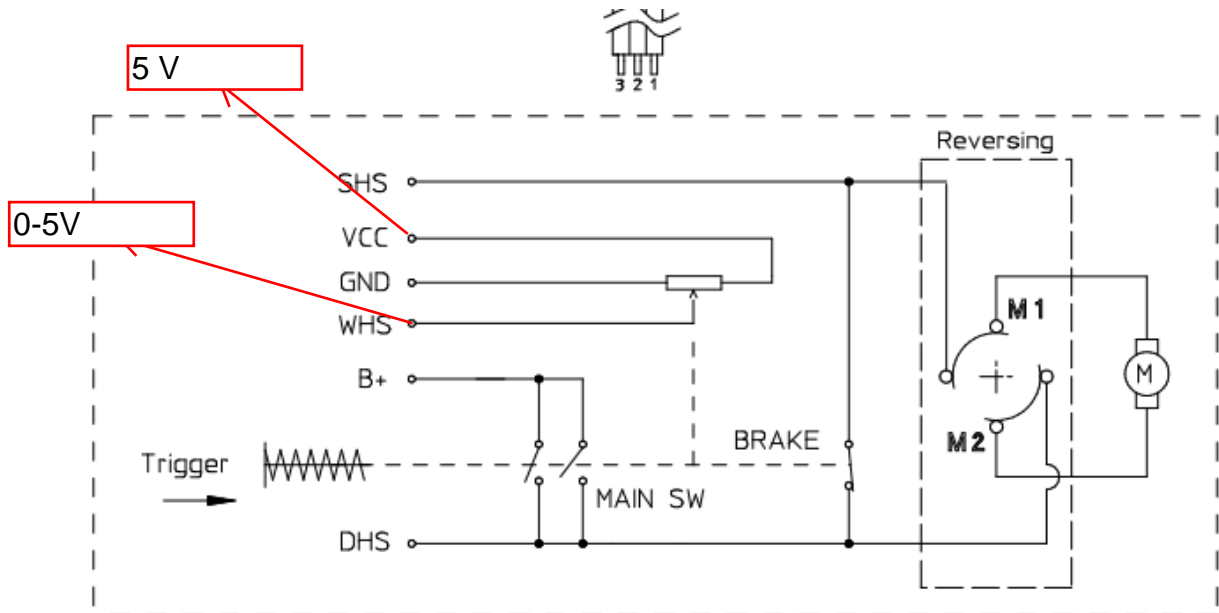
Circuit Schematic
