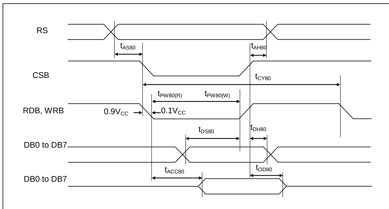
Figure 1. Read / Write Characteristics (8080-series MPU)
