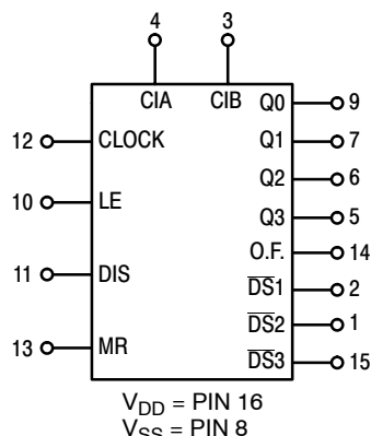
Figure 1. Block Diagram
