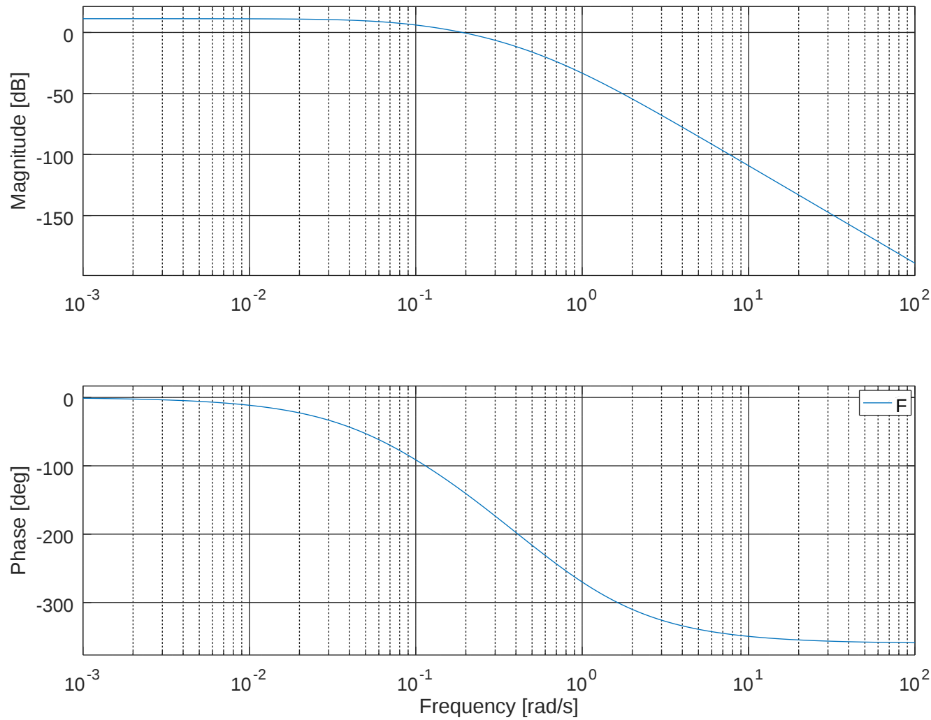
Bode Diagram
