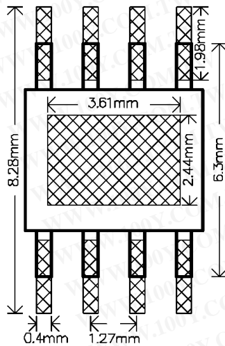
SOP-8 (FD)
