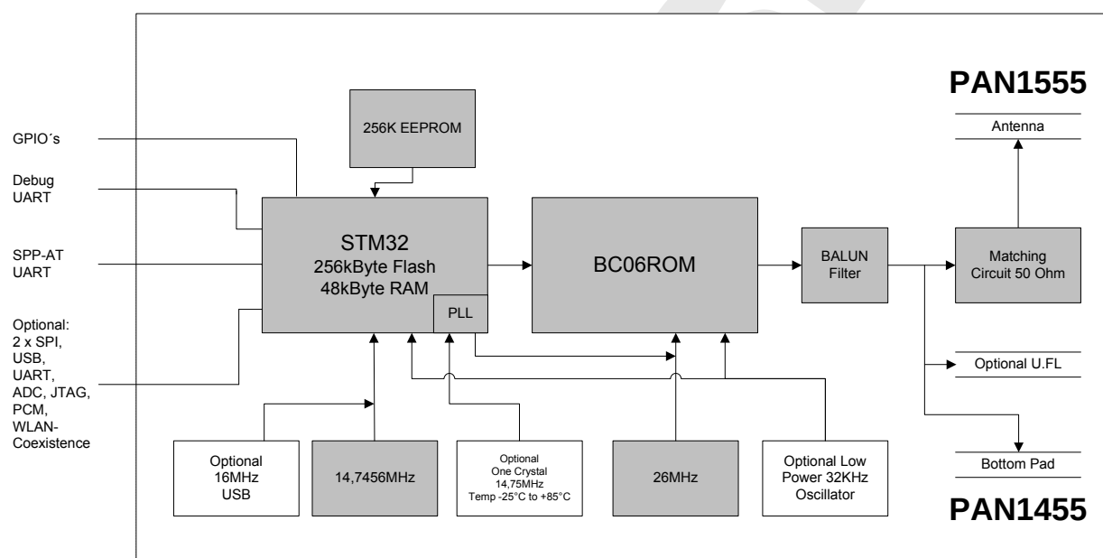
Figure 3.1 PAN1455/1555 Block-Diagram
