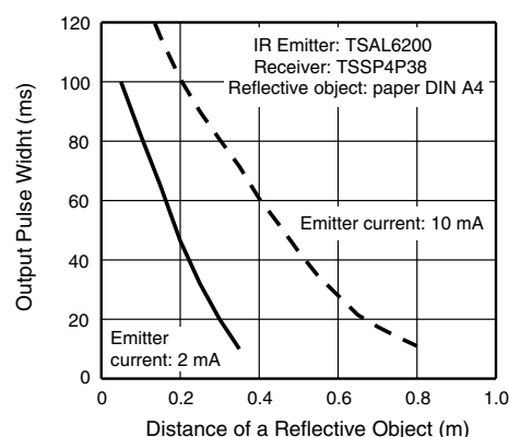
Fig. 13 - Distance Characteristic of a Typical Reflective Sensor Using the TSSP4P38
