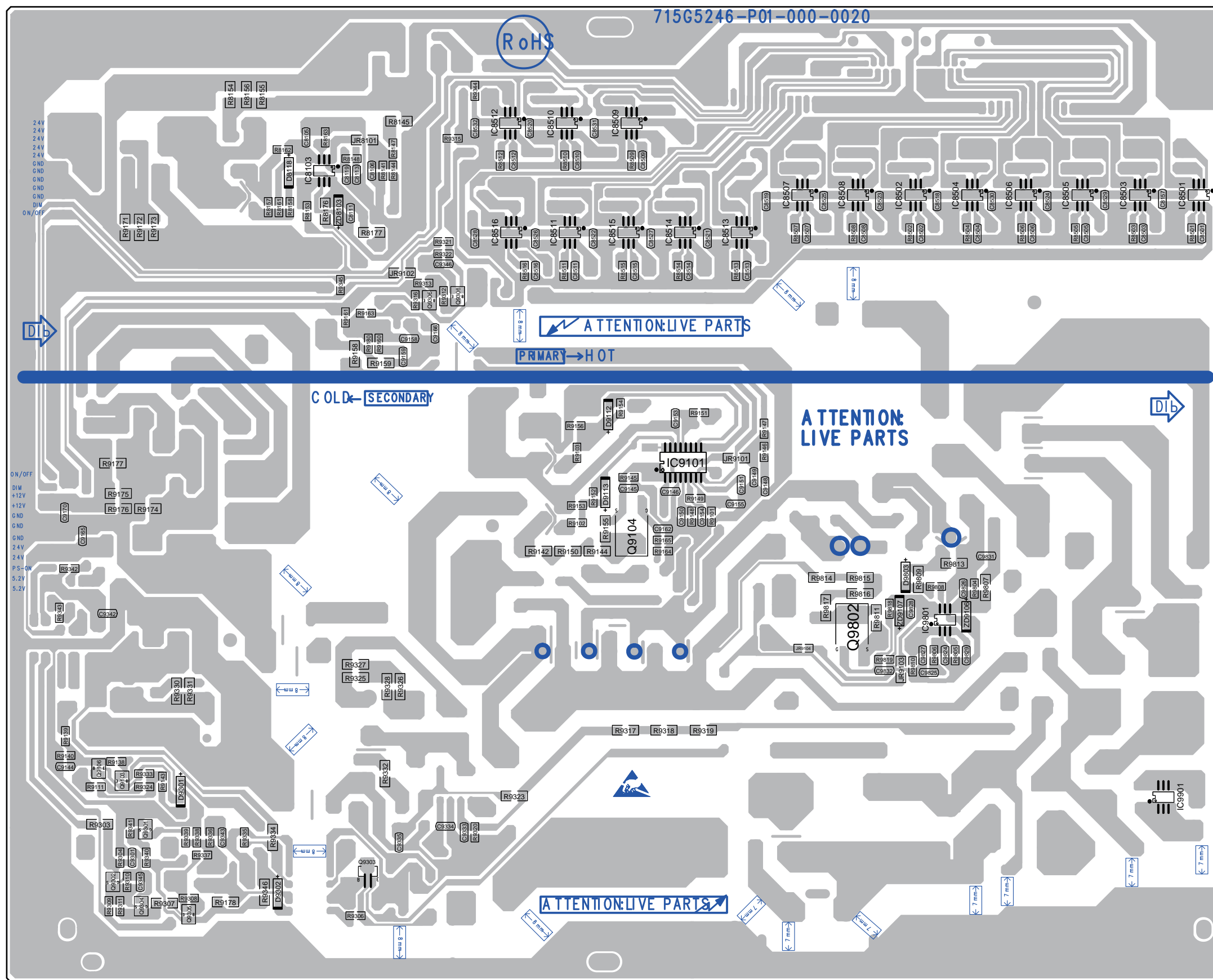
10-3-5 Power layout bottom
