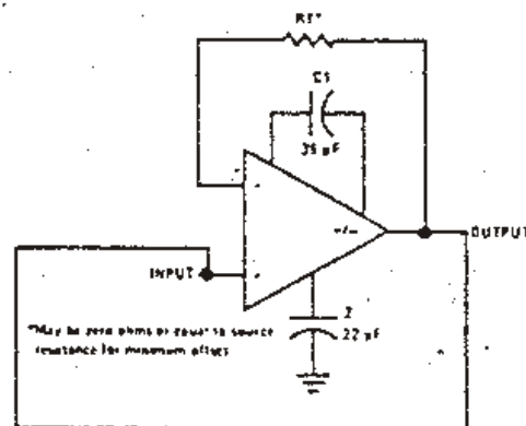
Voltage Follower
