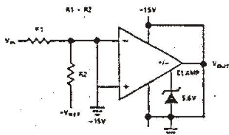
TTL/DTL Confusion Compounder
