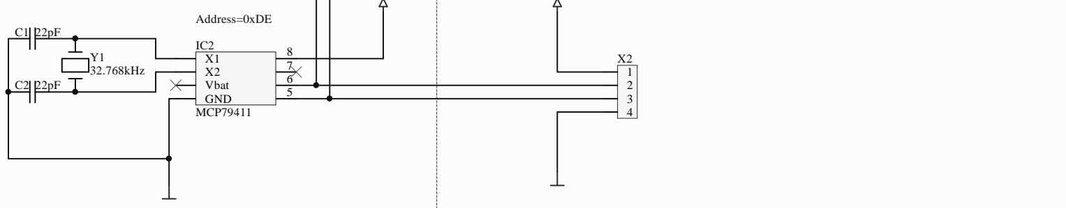
Real-Time-Clock (RTC)
