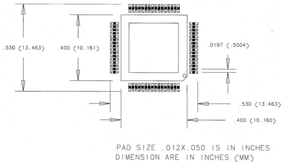
FIGURE 27. SUGGESTED FOOTPRINT
