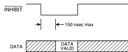
FIGURE 18. INHIBIT TIMING
