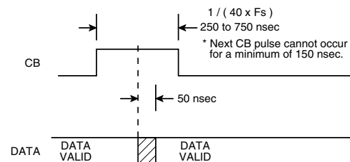
FIGURE 20. CONVERTER BUSY TIMING
