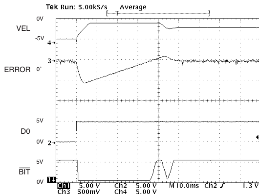
FIGURE 17. BENEFIT OF SWITCHING RESOLUTION ON THE FLY
