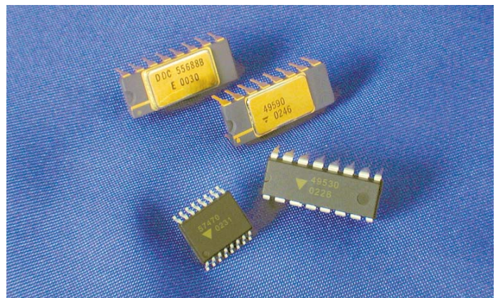
FIGURE 27. THIN-FILM RESISTOR NETWORKS
