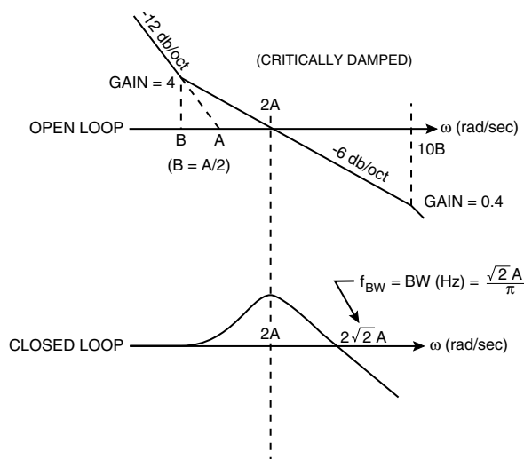
FIGURE 4. BODE PLOTS
