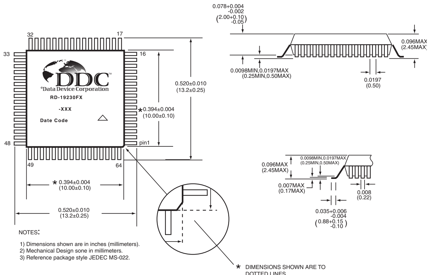
FIGURE 26. RD-19230 MECHANICAL OUTLINE (PLASTIC PACKAGE)
