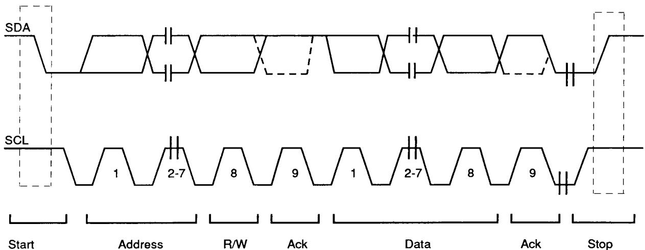
Figure 18. Data transfer on the Bus
