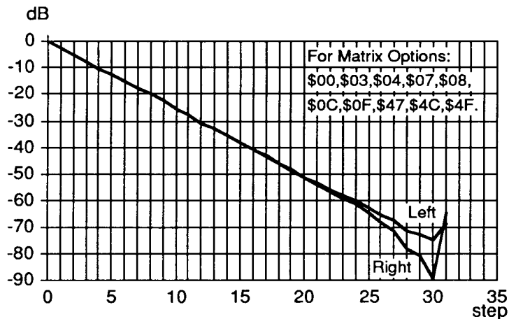
Figure 7: HP volume control
