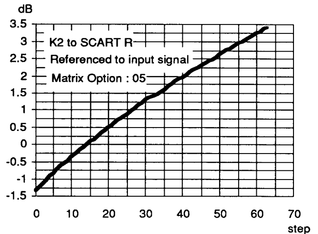
Figure 11: K2 set-up control
