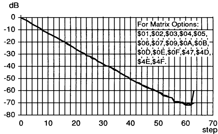
Figure 8: LS volume control
