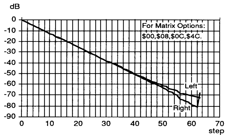
Figure 9: LS volume control
