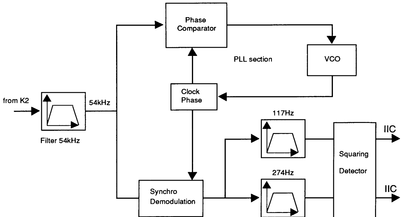
Figure 14. Pilot tone decoding
