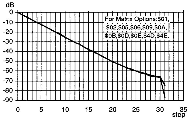
Figure 6: HP volume control
