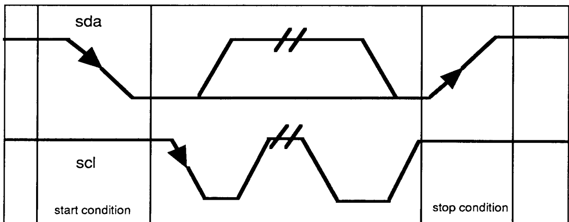
Figure 17. Start/Stop conditions
