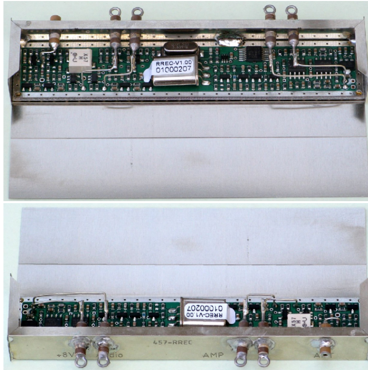
Figure 7: 457kHz Beacon Receiver PCB and front.
