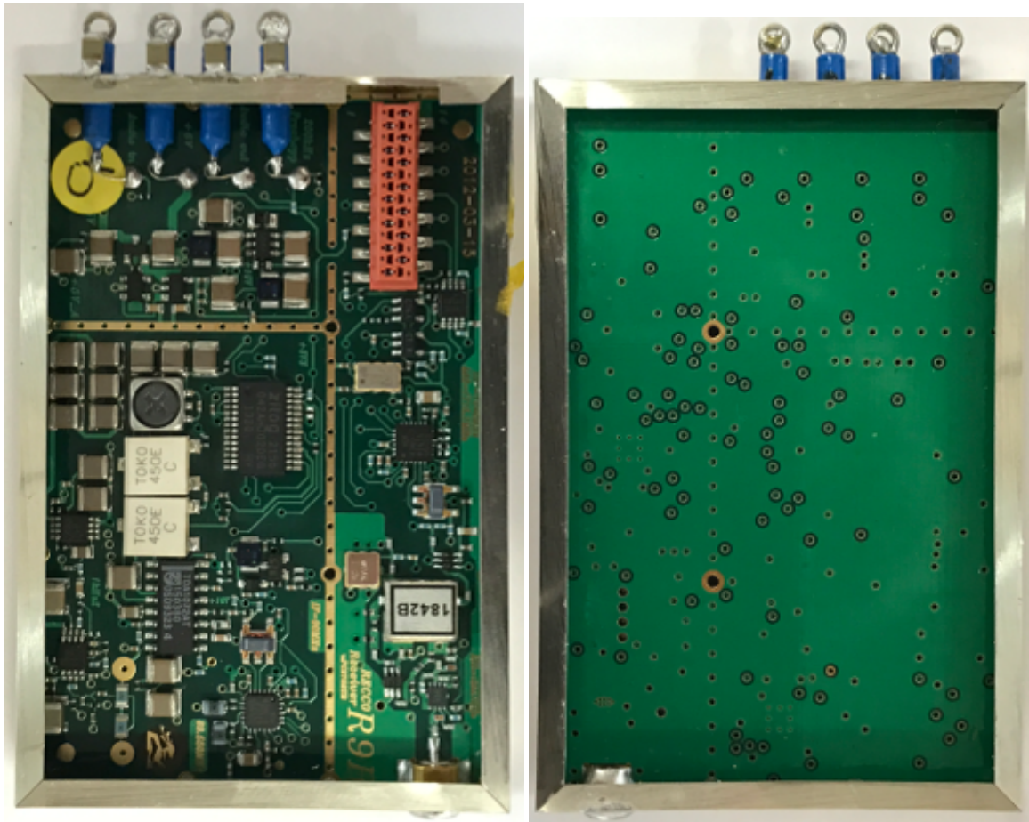
Figure 5: Recco Detector Rx PCB Top and Bottom sides.
