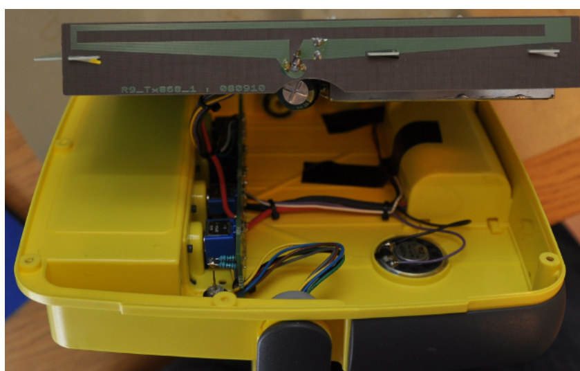
Figure 2: Recco Detector Internal Top. Showing the Tx antenna loop.
