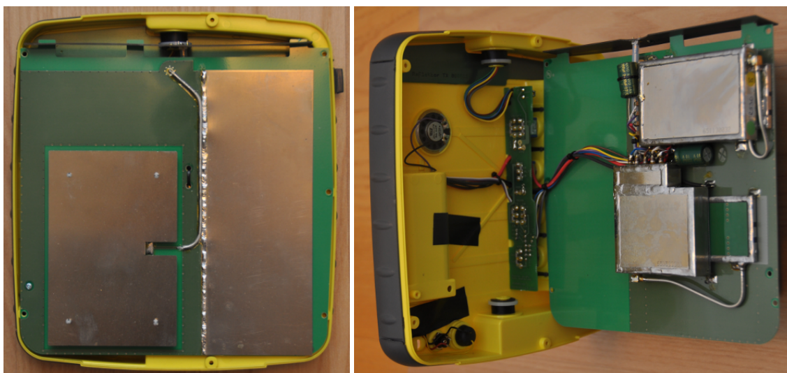
Figure 1: Recco Detector Internal Overview. (Left) Front side showing Rx and Tx antennas, (Right) Rear side showing loudspeaker, switch panel, headphone and charging connector. On the right showing Tx and Rx circuits and antenna backplane. Tx filter and Rx filter are located behind the shielded boxes
