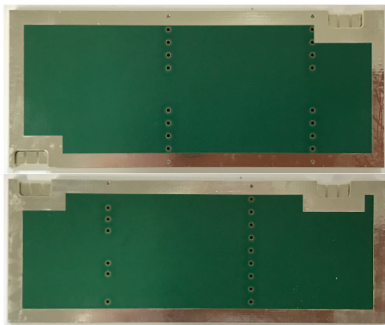
Figure 6: Recco Detector Tx and Rx output/input filters PCB. (PCB only no circuits).
