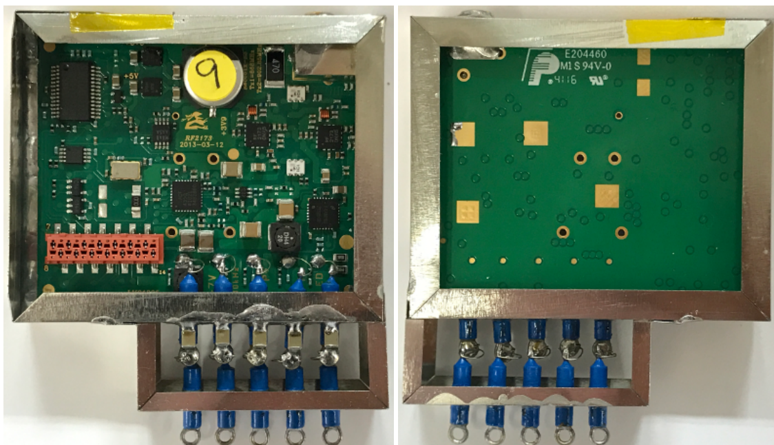
Figure 4: Recco Detector Tx PCB Top and Bottom sides.
