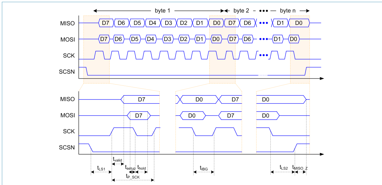
Figure 13. SPI timing
