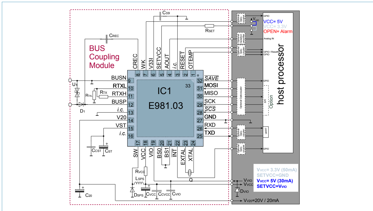
Figure 3. Schematic Example (full application)
