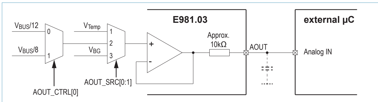
Figure 5. Analog Monitoring
