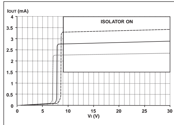
Fig. 5: Transconductance characteristic
