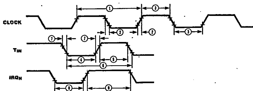
Figure 16. Additional Timing
