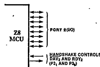
Figure 9c. Port 2
