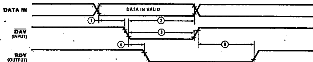
Figure 18a. Input Handshake
