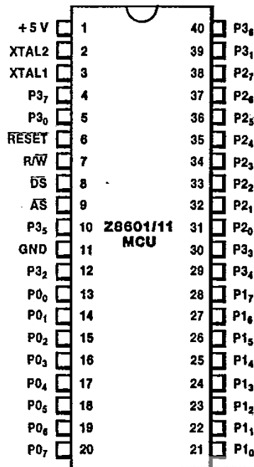
Figure 2a. 40-pin Dual-In-Line Package (DIP), Pin Assignments
