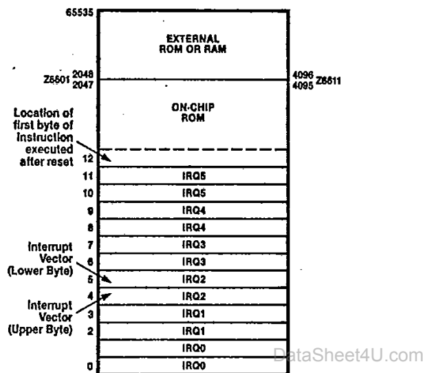
Figure 4. Program Memory Map
