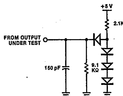
Figure 14. Test Load 1
