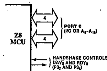
Figure 9b. Port 0
