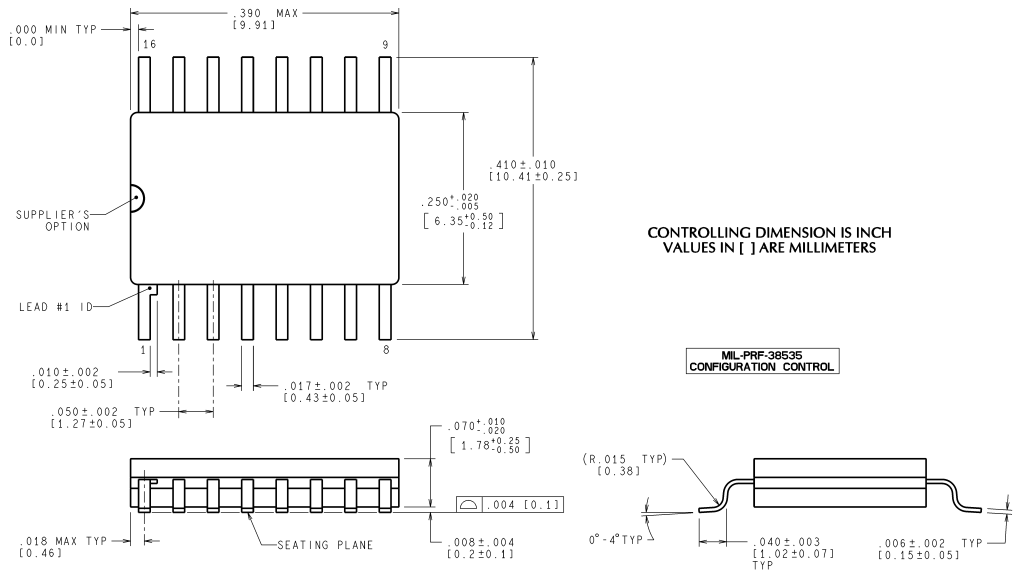
16 Lead Surface Mount Package (WG) See NS Package Number WG16A
