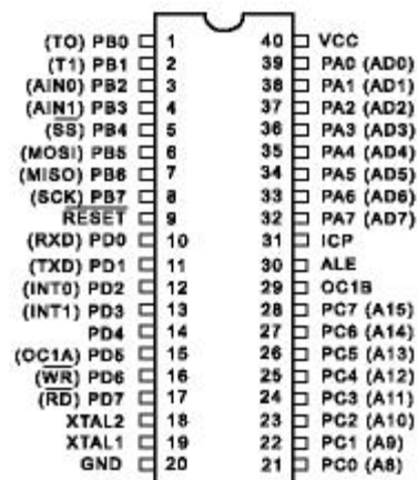
Abb. 3: Pin-Configuration des AT90S8515 (PDIP-Gehäuse)
