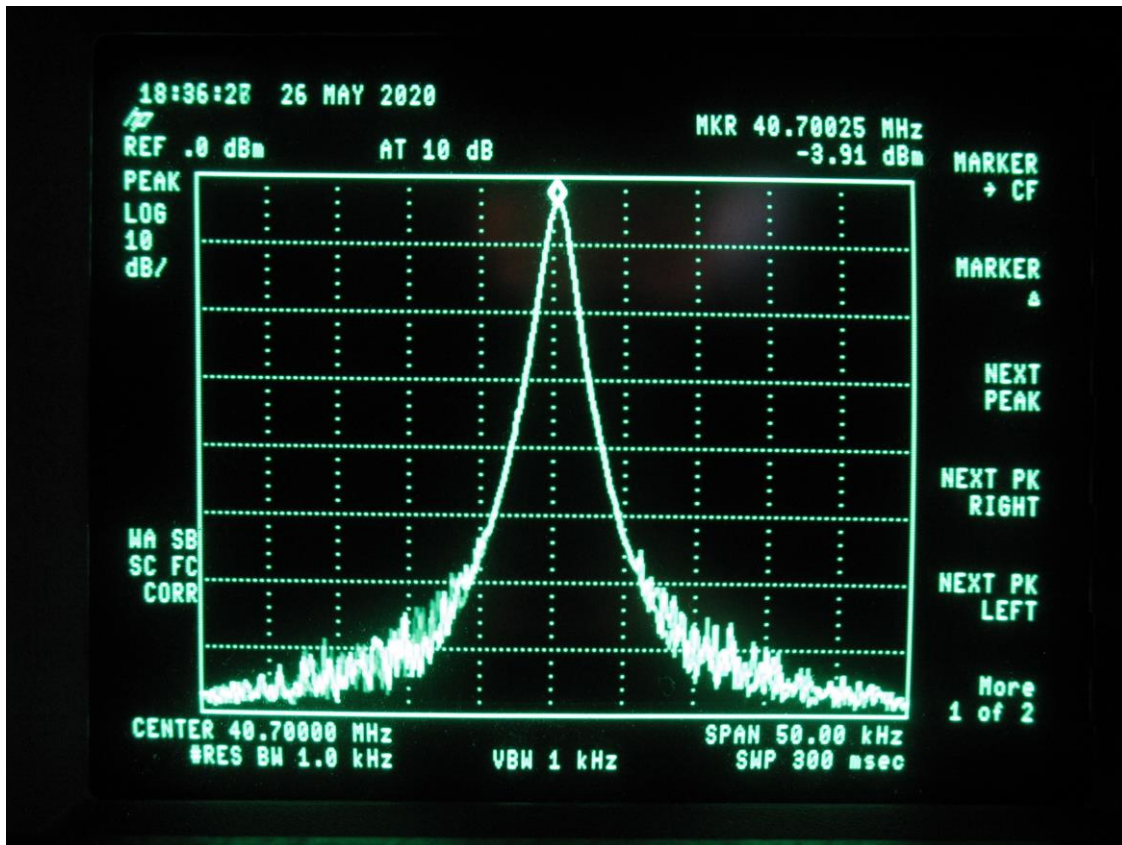
Span 50 kHz
