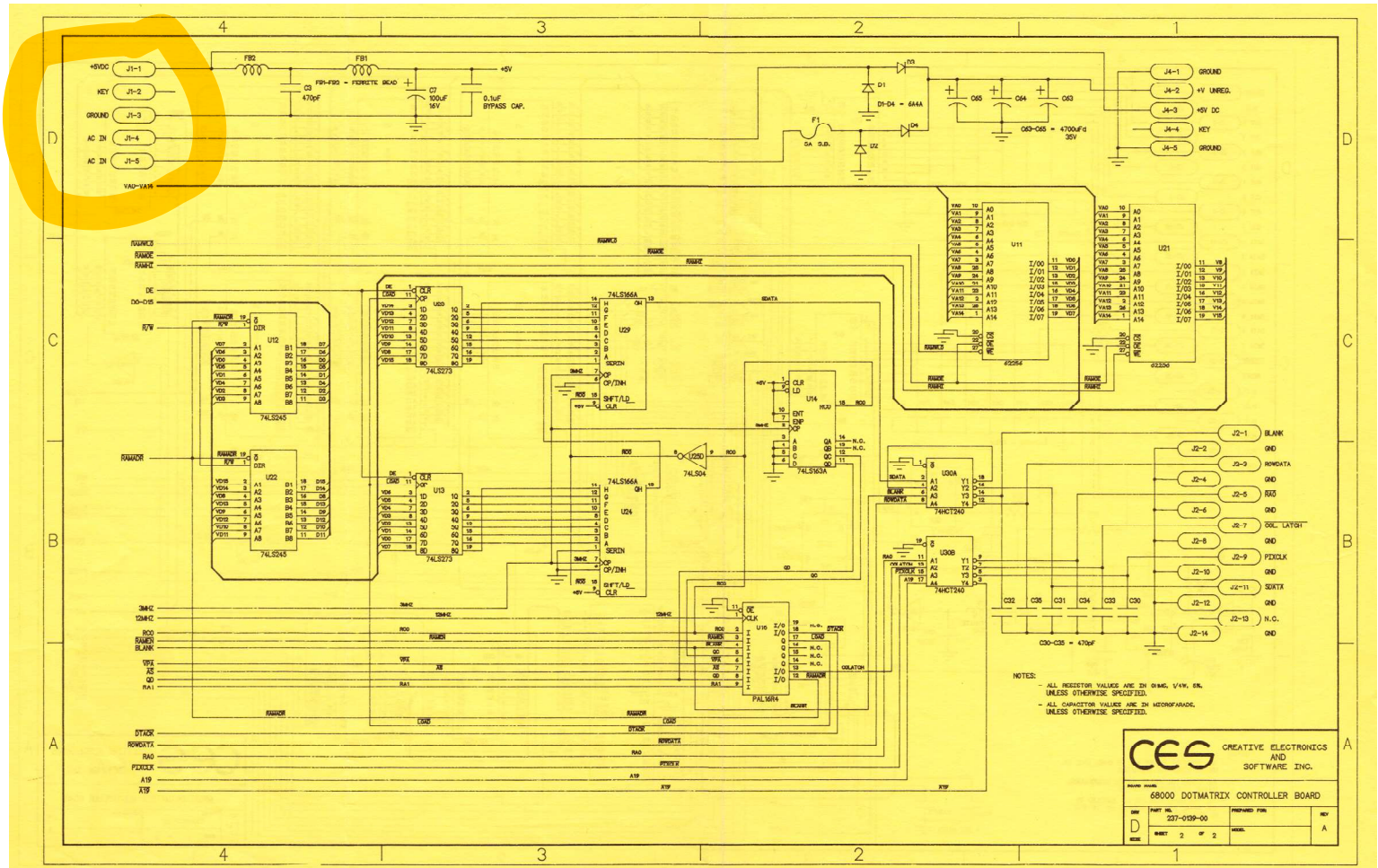
Display Controller Board Schematic (Page 2 of 2)
