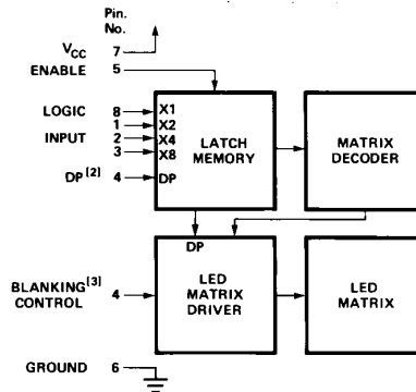
Figure 2. Block Diagram of 5082-7300 Series Logic.
