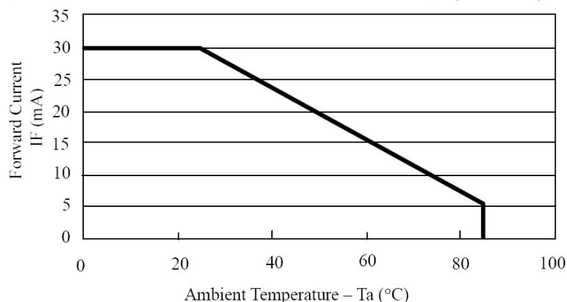
AMBIENT TEMP. VS. ALLOWABLE FORWARD CURRENT.(PER LED)
