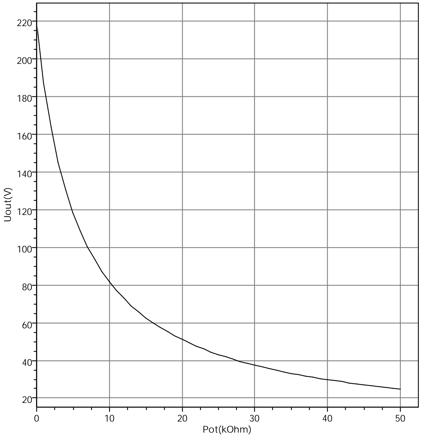
Uout of 25V-220V-Boost Module
