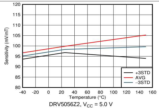
Figure 22. Sensitivity vs Temperature
