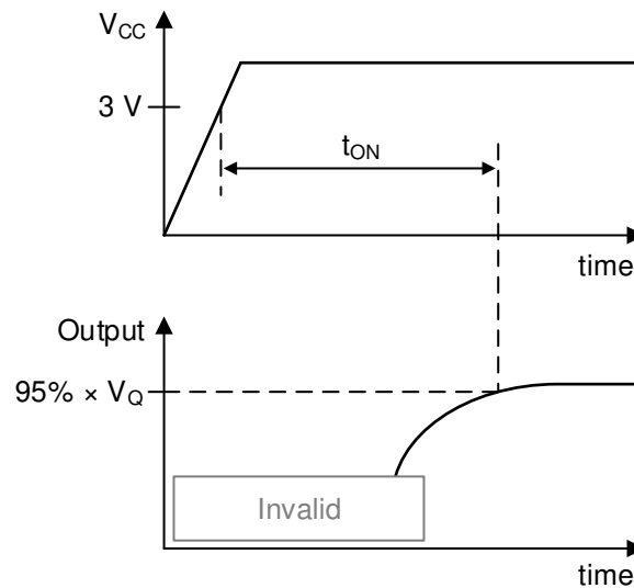
Figure 30. t_{ON} Definition
