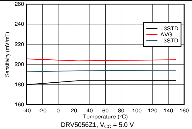
Figure 20. Sensitivity vs Temperature
