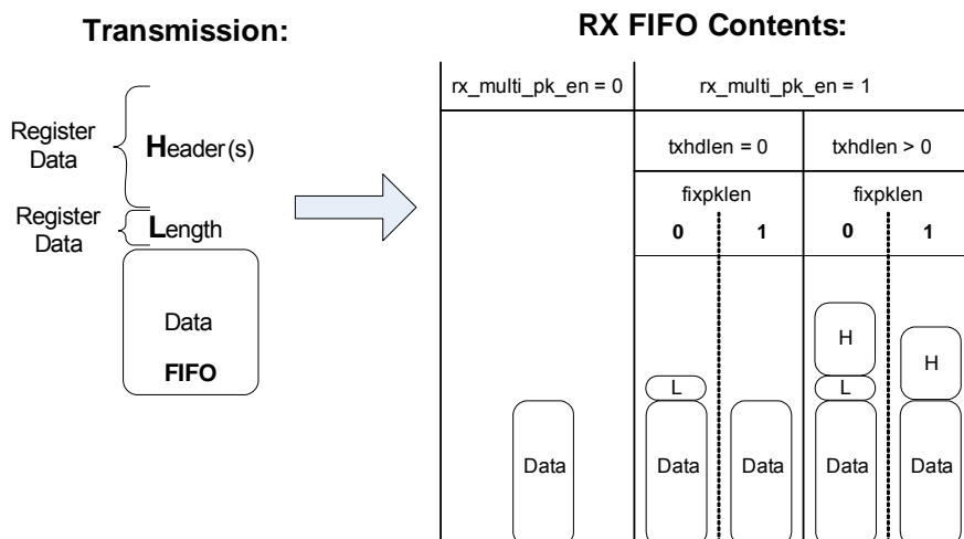
Figure 14. Multiple Packets in RX Packet Handler
