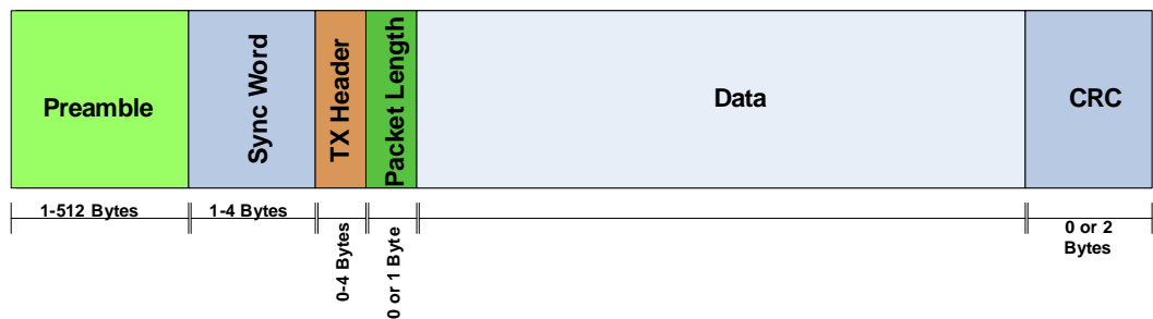
Figure 12. Packet Structure
