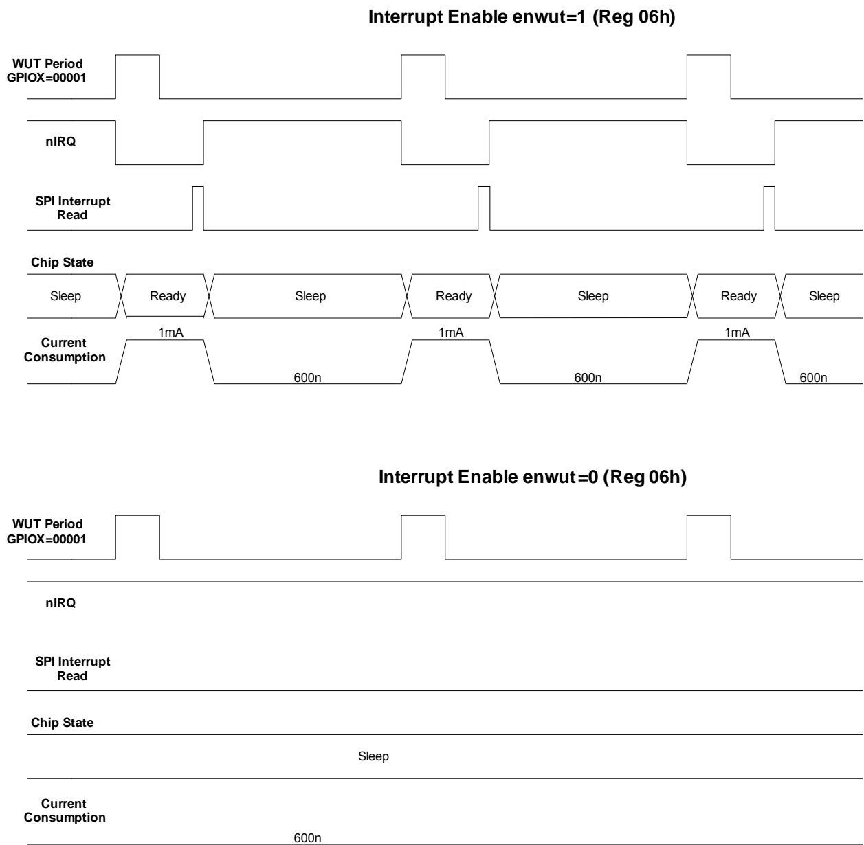
Figure 22. WUT Interrupt and WUT Operation
