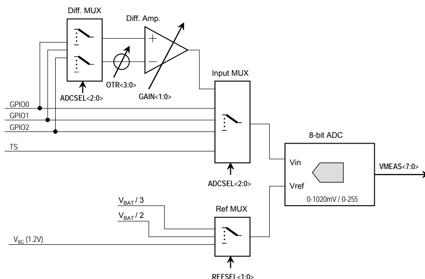
Figure 18. General Purpose ADC Architecture
