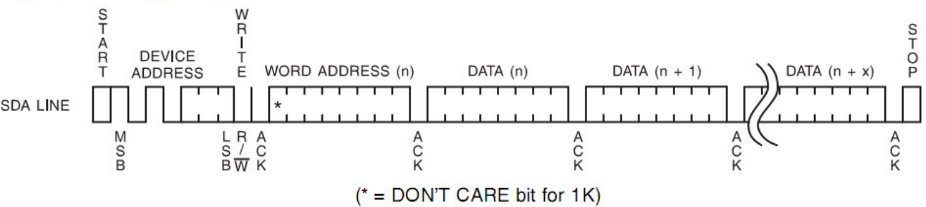
Figure 11-3. Page Write
