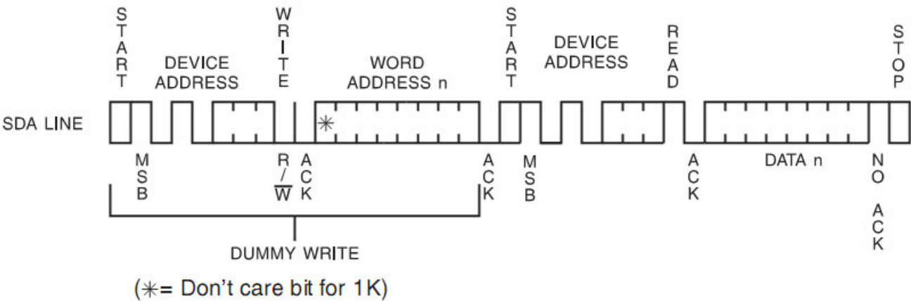
Figure 11-5. Random Read
