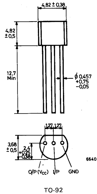
TO-92
