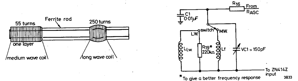
Coil winding details and waveband selection
