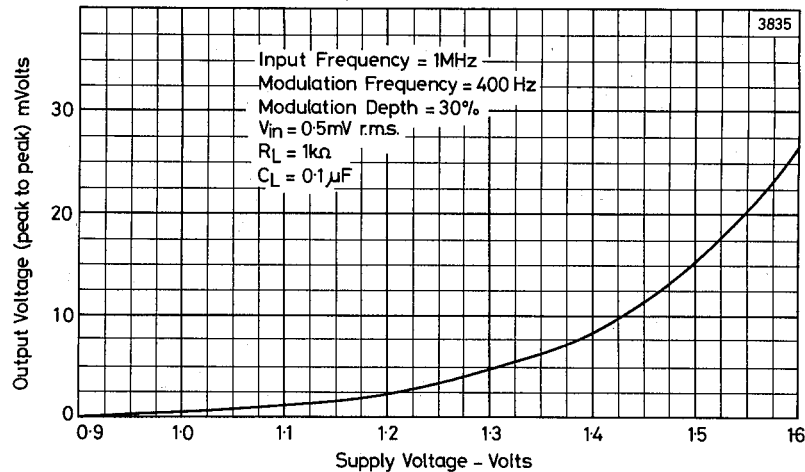
Gain variation with supply volts.
