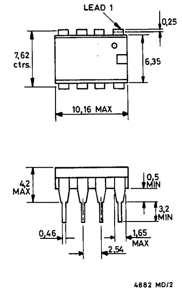
8 pin DIL
