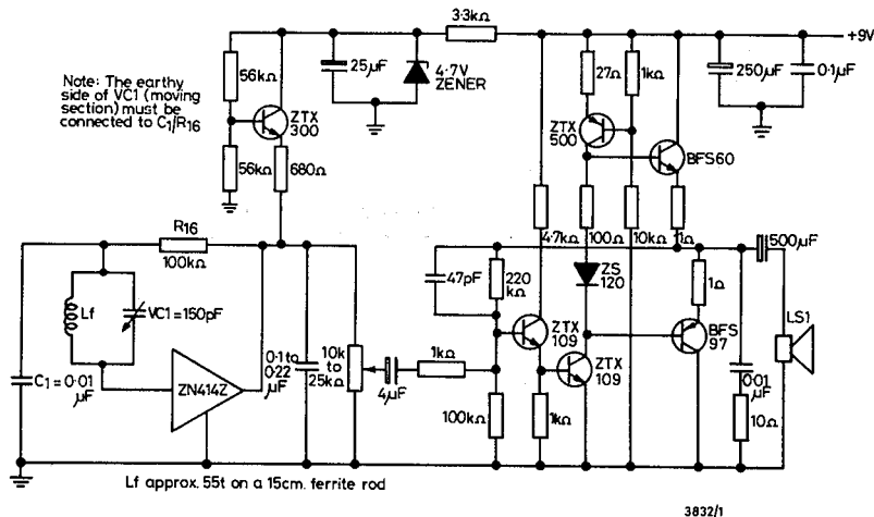
The complete circuit diagram of the Triffid receiver
