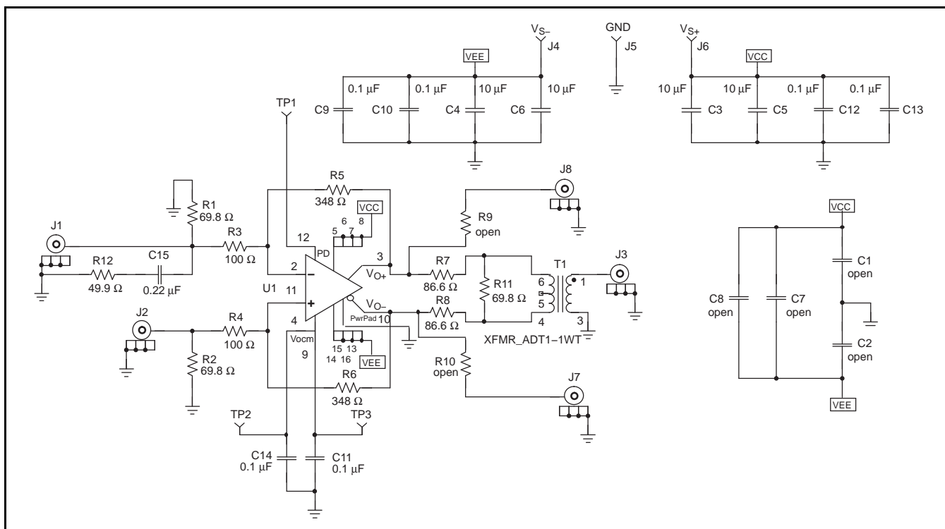
Figure 93. THS4509 EVAL1 EVM Schematic
