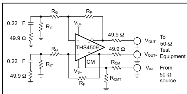
Figure 79. CM Input Test Circuit
