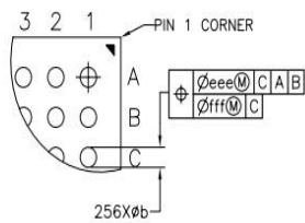
DETAIL B(2:1)
