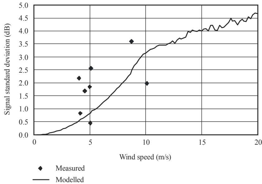
FIGURE 8 Standard deviation of measured and modelled 40 GHz time series as a function of wind speed
