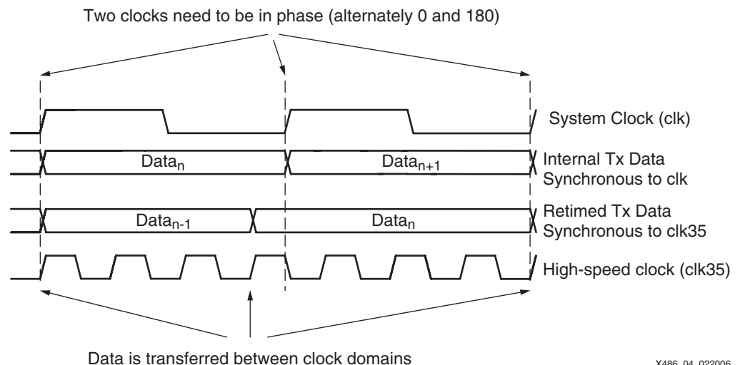
Figure 5: Internal Timing for Logic Version
