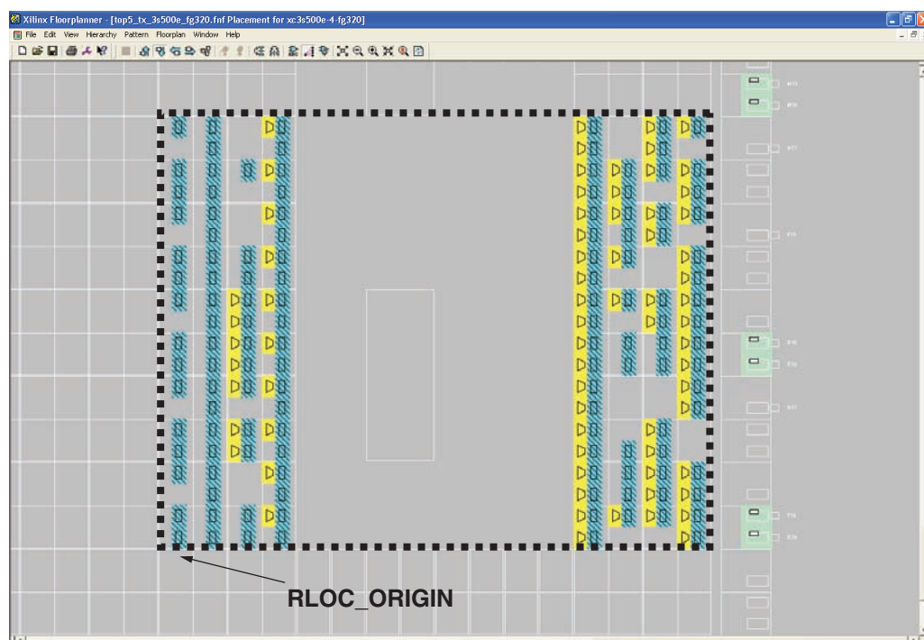
Figure 9: 5-Bit Spartan-3E Transmitter Macro
