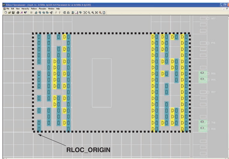
Figure 8: 4-Bit Spartan-3E Transmitter Macro
