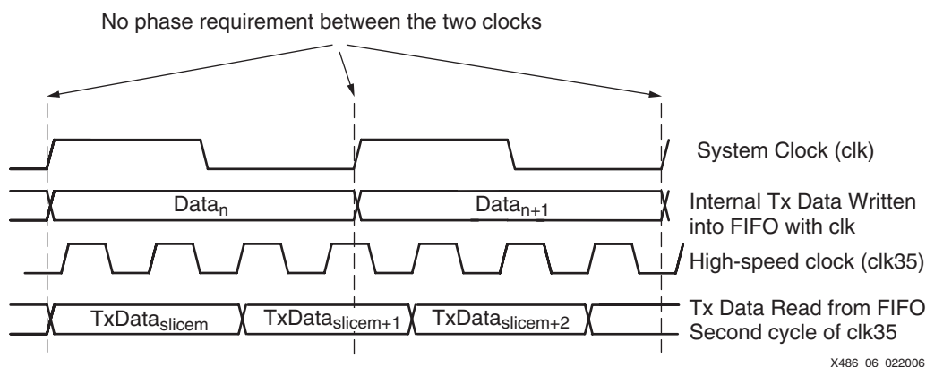
Figure 7: Internal Timing for FIFO Version
