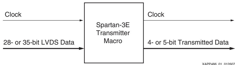
Figure 1: 7:1 Transmitter Module
