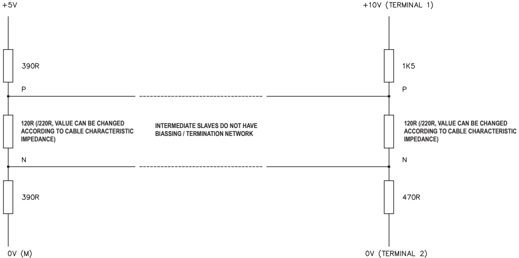
MM4 RS485 (USS) TERMINATION/ BIASING NETWORKS
