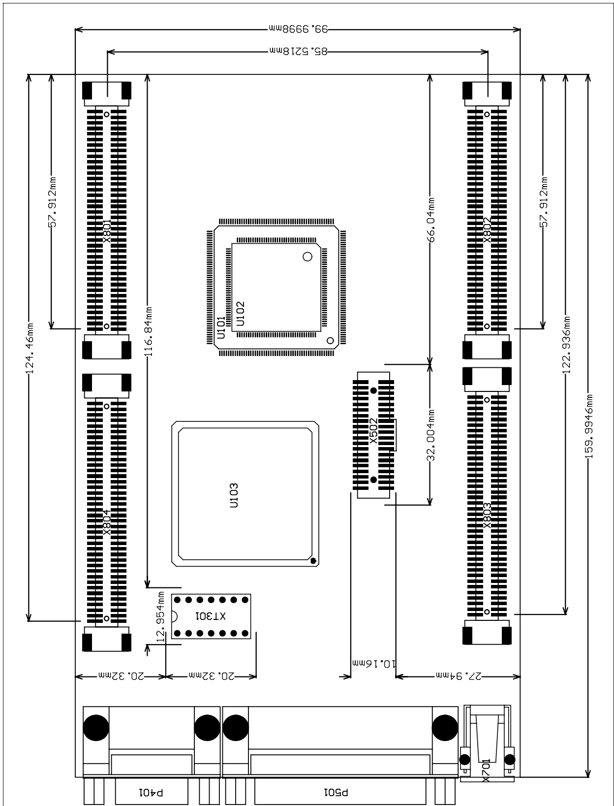
Figure 8-14 Dimensioning (mm)
