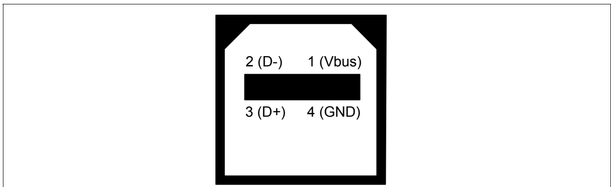
Figure 7-6 USB connector Pinout
