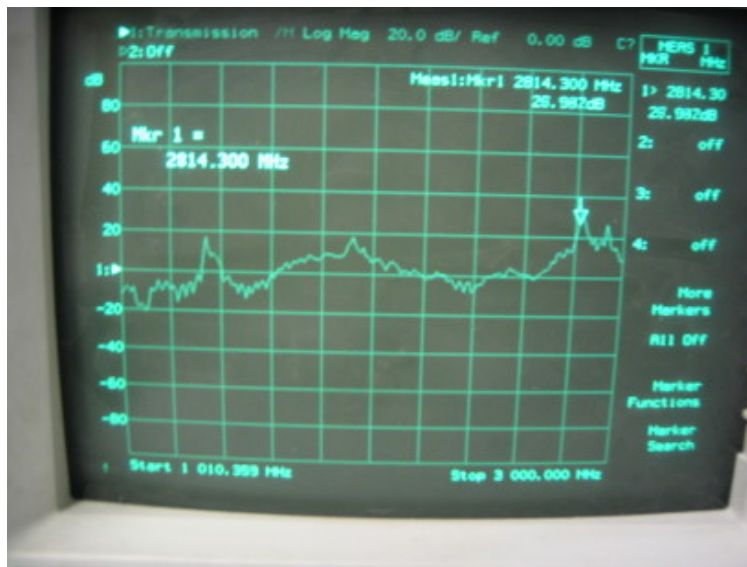
A typical attenuation trace form the network analyser
