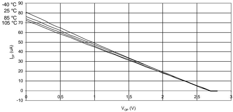
Figure 27-12. I/O Pin Pull-Up Resistor Current vs. Input Voltage ( V_{CC} = 2.7V ) I/O PIN (including PE1 & PE2) PULL-UP RESISTOR CURRENT vs. INPUT VOLTAGE V_{CC} = 2.7 V
