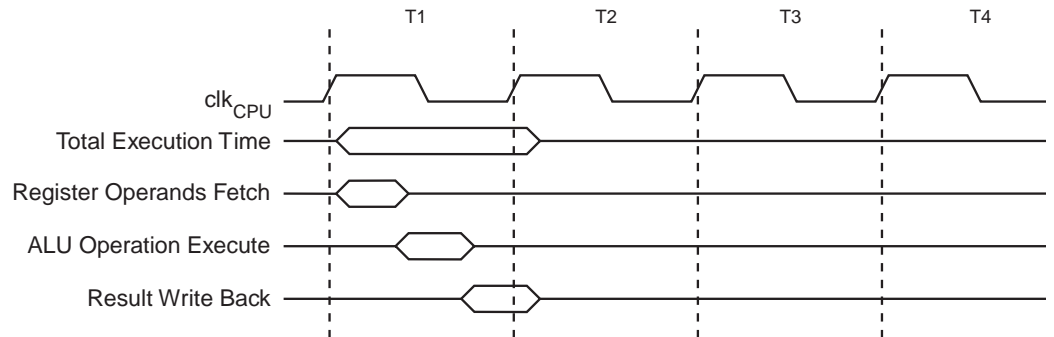
Figure 5-5. Single Cycle ALU Operation
