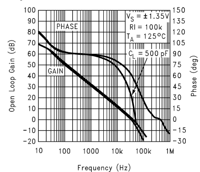
Gain and Phase vs Capacitive Load @ 2.7V
