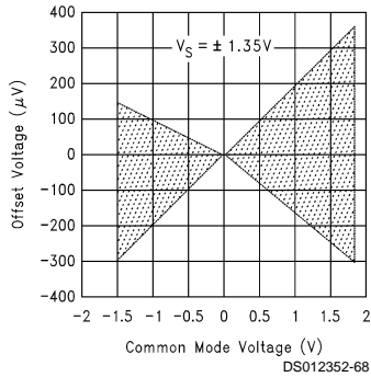
Offset Voltage vs Common Mode Voltage @ 2.7V
