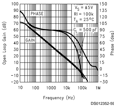
Gain and Phase vs Capacitive Load @ 10V
