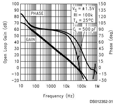
Gain and Phase vs Capacitive Load @ 3V
