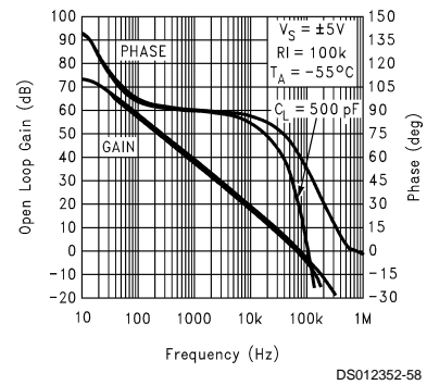
Gain and Phase vs Capacitive Load @ 10V
