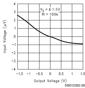
Output Voltage vs Input Voltage @ 3V
