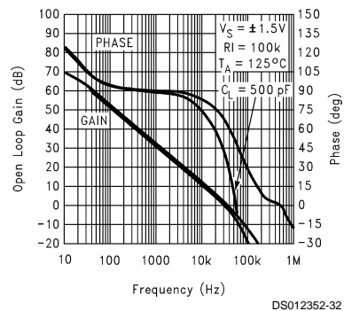
Gain and Phase vs Capacitive Load @ 3V
