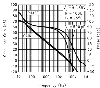
Gain and Phase vs Capacitive Load @ 2.7V
