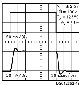
Non-Inverting Small Signal Pulse Response at 5V
