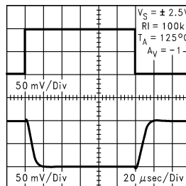
Inverting Small Signal Pulse Response at 5V
