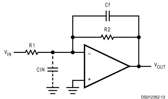
FIGURE 3. Cancelling the Effect of Input Capacitance
