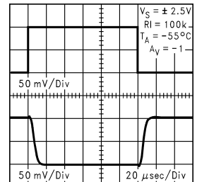
Inverting Small Signal Pulse Response at 5V
