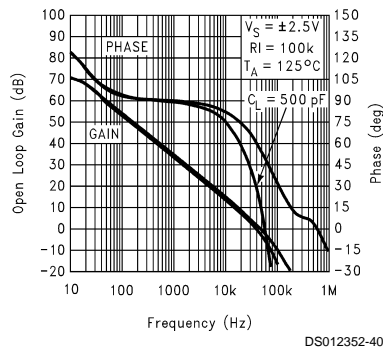
Gain and Phase vs Capacitive Load @ 5V
