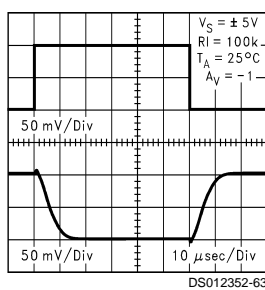
Inverting Small Signal Pulse Response at 10V
