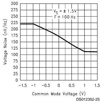
Voltage Noise vs Common Mode Voltage @ 3V
