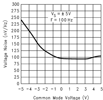
Voltage Noise vs Common Mode Voltage @ 10V
