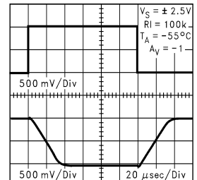
Inverting Large Signal Pulse Response at 5V
