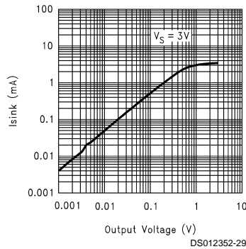
Sinking Output vs Output Voltage
