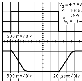
Inverting Large Signal Pulse Response at 5V
