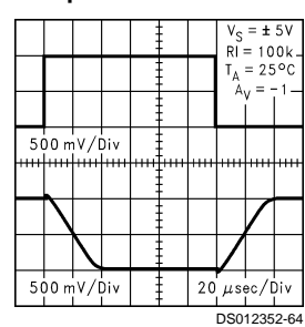
Inverting Large Signal Pulse Response at 10V
