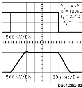
Non-Inverting Large Signal Pulse Response at 10V
