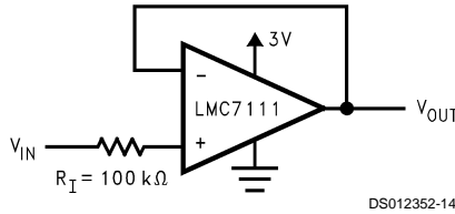
FIGURE 1. R_I Input Current Protection for Voltages Exceeding the Supply Voltage
