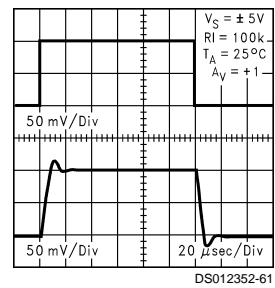
Non-Inverting Small Signal Pulse Response at 10V
