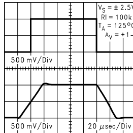
Non-Inverting Large Signal Pulse Response at 5V
