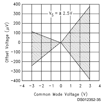
Offset Voltage vs Common Mode Voltage @ 5V
