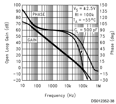
Gain and Phase vs Capacitive Load @ 5V
