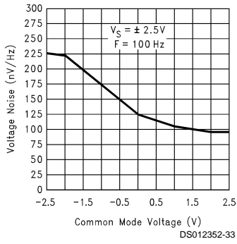
Voltage Noise vs Common Mode Voltage @ 5V
