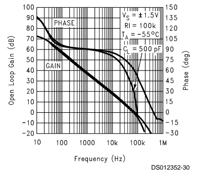
Gain and Phase vs Capacitive Load @ 3V
