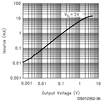
Sourcing Output vs Output Voltage
