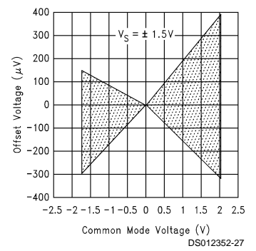
Offset Voltage vs Common Mode Voltage @ 3V
