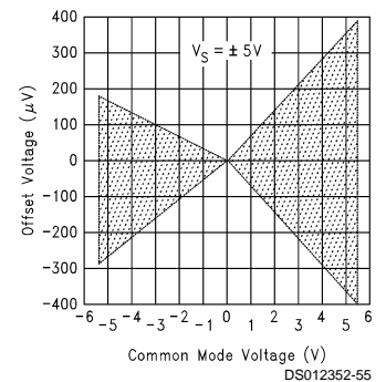
Offset Voltage vs Common Mode Voltage @ 10V
