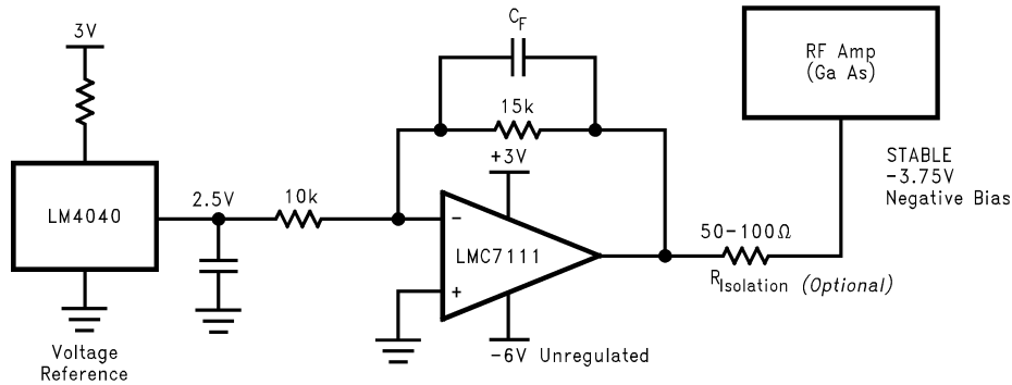
FIGURE 4. Stable Negative Bias
