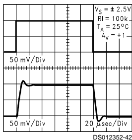
Non-Inverting Small Signal Pulse Response at 5V
