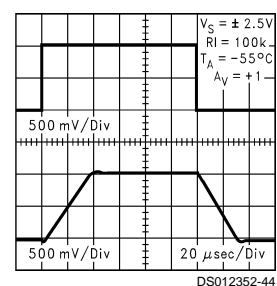
Non-Inverting Large Signal Pulse Response at 5V
