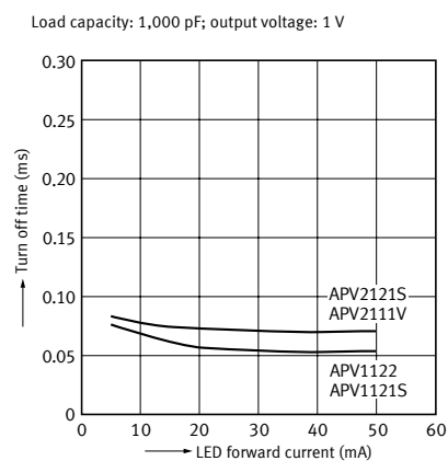
9. Turn off time vs. LED forward current characteristics
