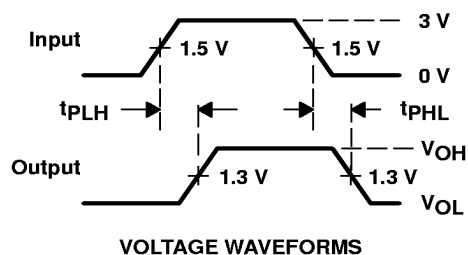
Figure 3. Driver Test Circuit and Voltage Waveforms
