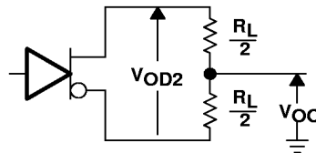
Figure 1. Driver V_{OD2} and V_{OC}
