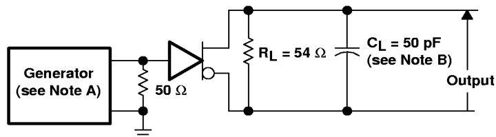
TEST CIRCUIT
