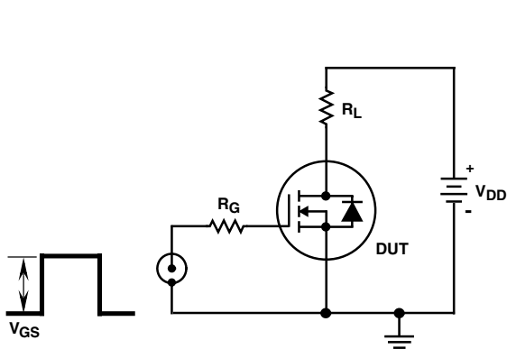
FIGURE 14. SWITCHING TIME TEST CIRCUIT
