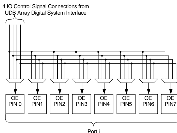
Figure 7-17. I/O Pin Output Enable Connectivity
