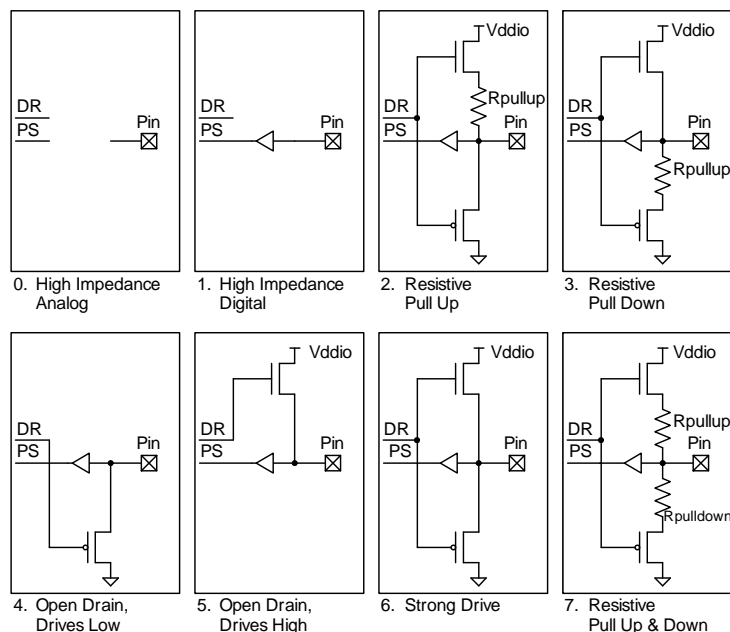
Figure 6-9. Drive Mode
