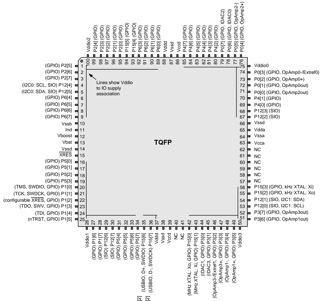
Figure 2-3. 100-Pin TQFP Part Pinout
