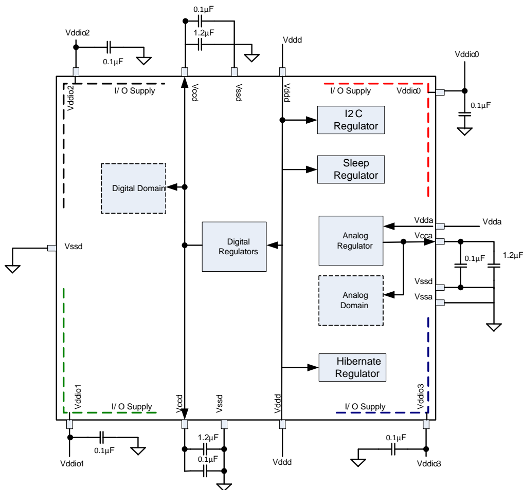
Figure 6-2. PSoC Power System
