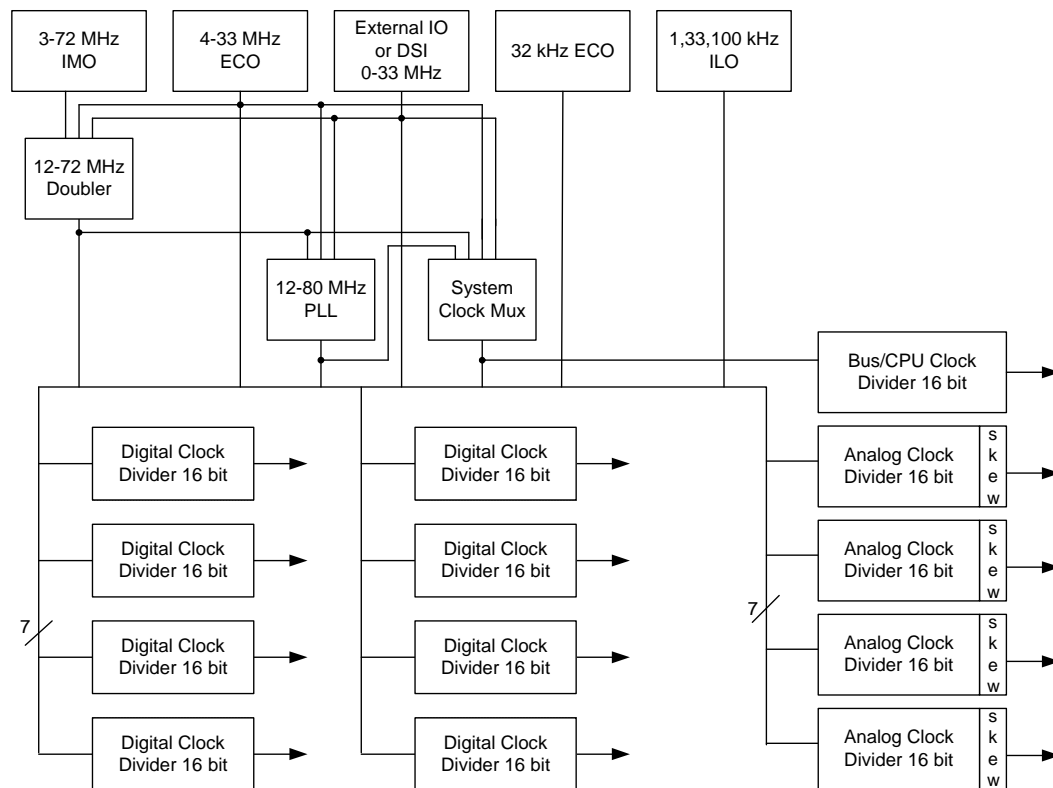
Figure 6-1. Clocking Subsystem
