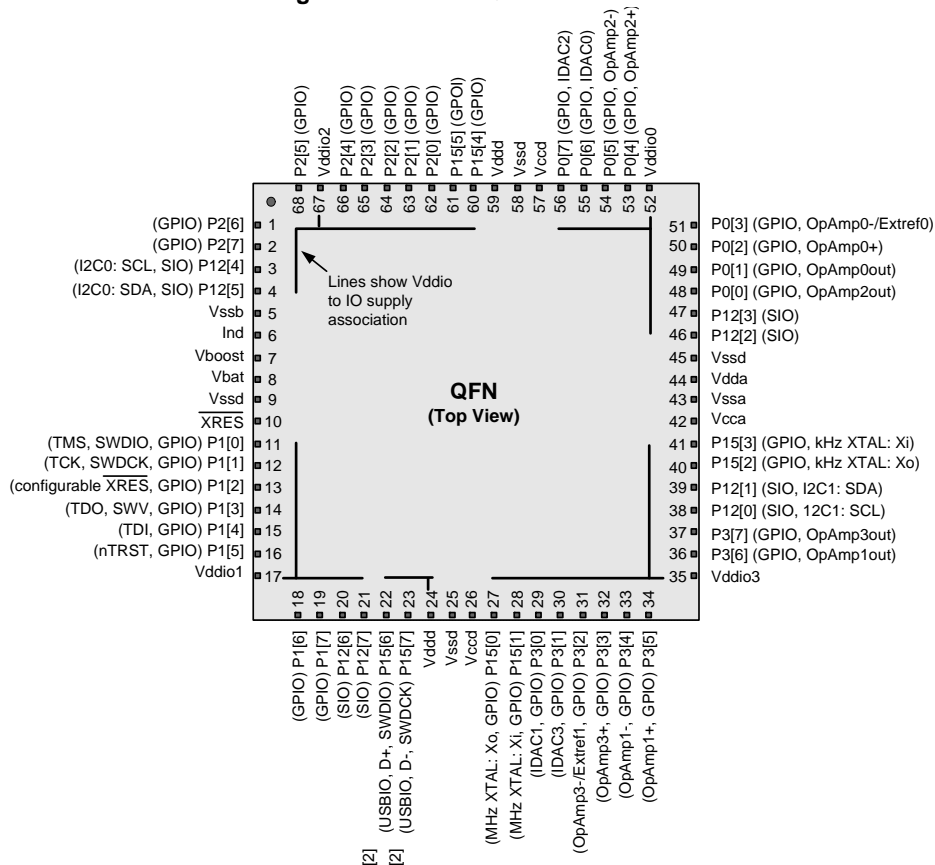
Figure 2-2. 68-Pin QFN Part Pinout
