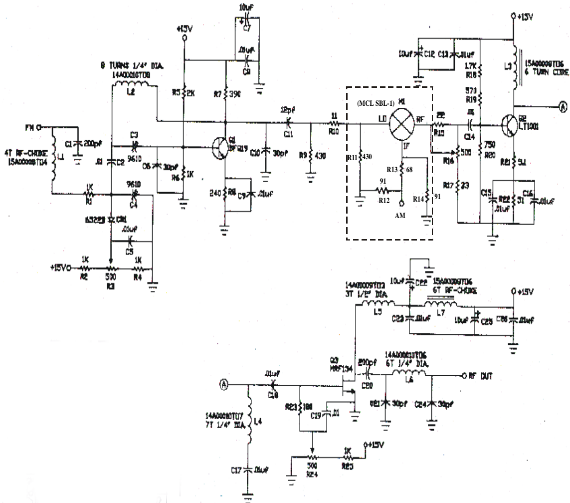
Figure 6.1: The circuit diagram of a NEOS acousto optic modulator RF driver (NEOS model N21080-1AMVCO). The dashed rectangle indicates the components that were missing in our AOM driver (NEOS model N21060-1.5M) and needed for AM input construction.
