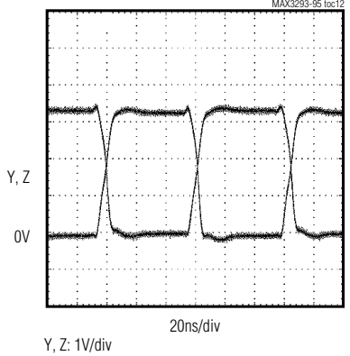
UNLOADED DRIVER OUTPUT WAVEFORM ( f_{IN} = 16Mbps )
