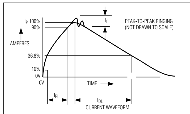
Figure 11. Current Waveform
