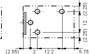
Mounting Holes (Bottom View) Tolerance: \pm 0.1\text{mm}
