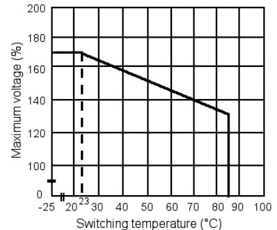
Ambient Temp. Vs Max. Voltage
