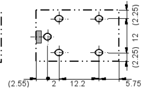
Mounting Holes (Bottom View) Tolerance: \pm 0.1\text{mm}
