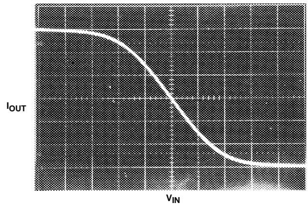
FIGURE 3B. WITH DIODE PROGRAMMING TERMINAL CUTOFF
