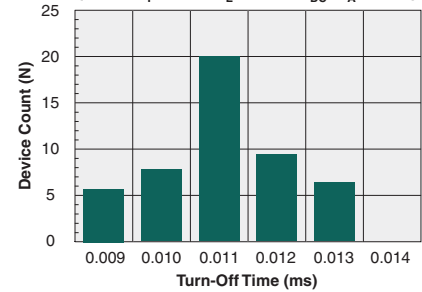
Typical Turn-Off Time (N=50, I_F=5\text{mA} , I_L=120\text{mA}_{DC} , T_A=25^\circ\text{C} )
