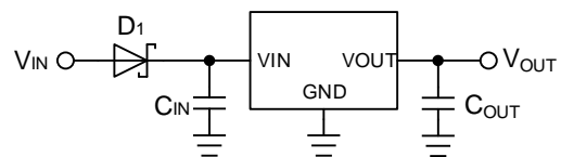
Figure 30. Protection against Reverse Polarity 1
